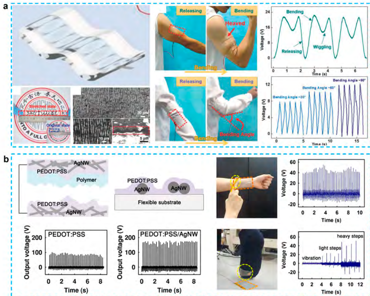
Figure 8. (a) A wrinkled PEDOT:PSS film-based stretchable and transparent triboelectric nanogenerator for wearable energy harvesters and active motion sensors [107]. (b) Transparent and flexible high power triboelectric nanogenerator with metallic nanowire-embedded tribonegative conducting polymer [101].
