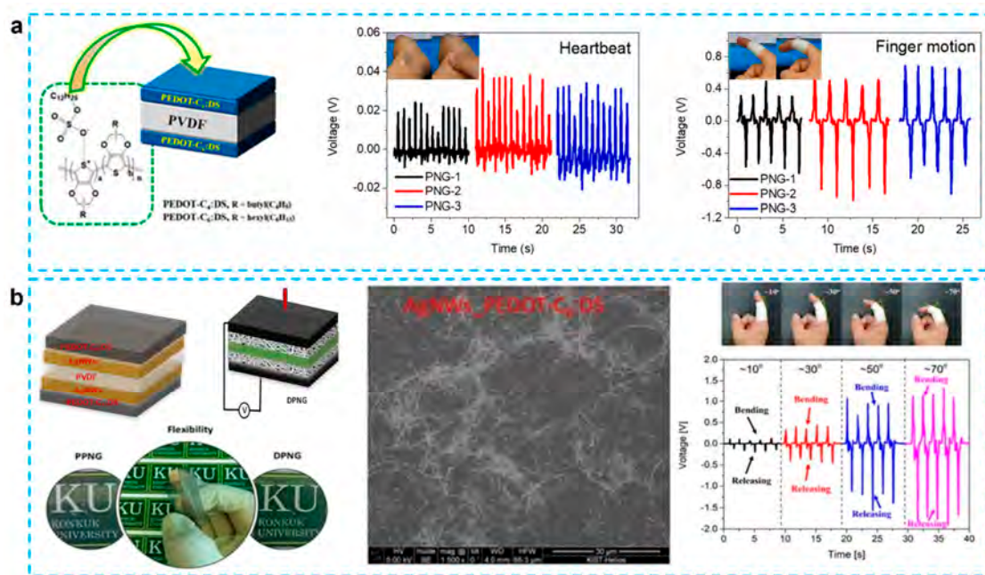
Figure 5. (a) Schematic illustration of sandwich structure with PEDOT-Cx:DS. The generated output voltage performance from the PNGs used for heartbeat monitoring system attached to wrist and human motion monitoring system attached to index finger [59]. (b) Schematics of DPNG, Photographs of transparency of AgNWs film, Flexible PVDF based hybrid electrode PNG and transparency of hybrid electrode, cross-section SEM images of DPNG, Performance of flexible DPNG under index finger movement [26].
